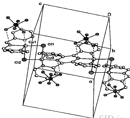
Figure 2 Cell drawing of the complex, [\{\text{CuCl}\}_2(\mu\text{-tpzz})](\text{PF}_6)_2 . Selected bond lengths (Å) and bond angles (deg): Cu2-Cl2, 2.2431(12); Cu1-Cl2, 2.7196(13); Cu1-Cl2-Cu2, 83.20(4); Cl1-Cu1-Cl2, 96.80(4).
