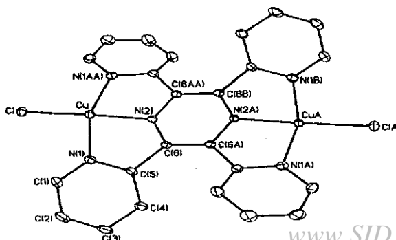
Figure 1 ORTEP of the complex, [\{CuCl\}_2(\mu\text{-tppz})](PF_6)_2 , the counter anions have been excluded for clarity.
