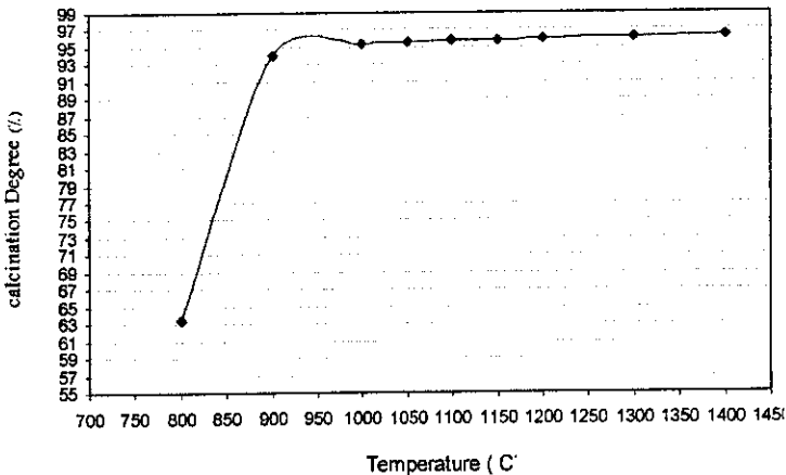
Figure 5 Shahreza dolomite calcination degree – temperature relationship.
