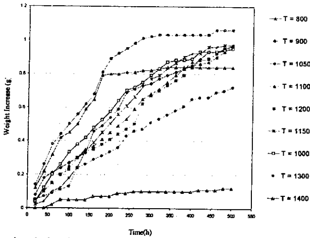
Figure 8 Hydration behavior of Shahreza dolomite calcined at various temperatures.
