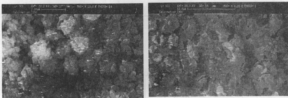
Figure 6 Secondary electron images of the Shahreza dolomite calcined at (a) 1150 °C and (b) 1400 °C.
