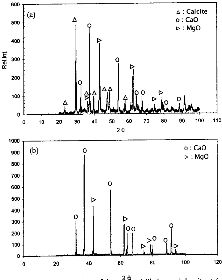
Figure 4 X-ray diffraction patterns of the calcined Shahreza dolomite at (a) 800 °C and (b) 1100°C
