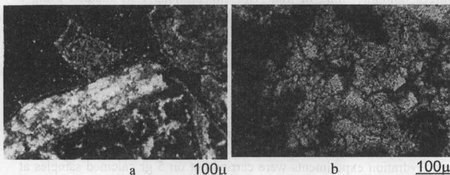
Figure 1 photo microscoph of the Shahreza dolomite ore indicating (a) a calcite veinlet (white lath), and (b) iron rich regions (dark areas).
