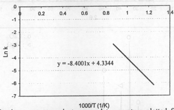
Figure 7 Kinetics constant against reversed temperature plotted for fine dolomite particles.
