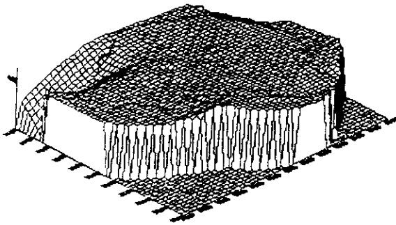
Shepard,s Method
