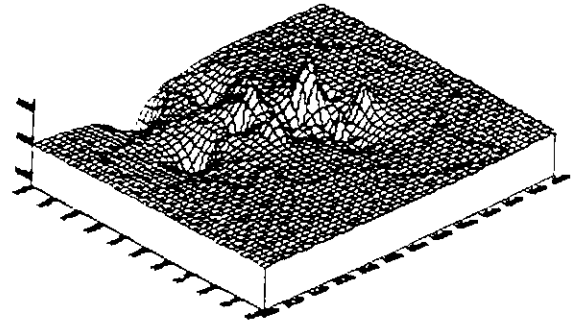
Invers Distance to a power Method
