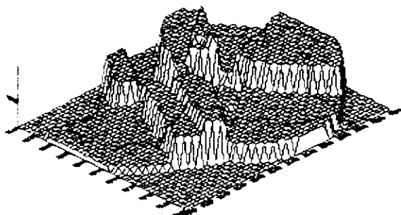
Nearest Neighbor Method
