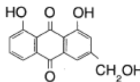
Aloe-emodin
