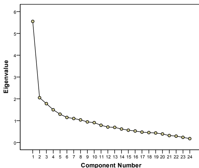
Scree Plot
