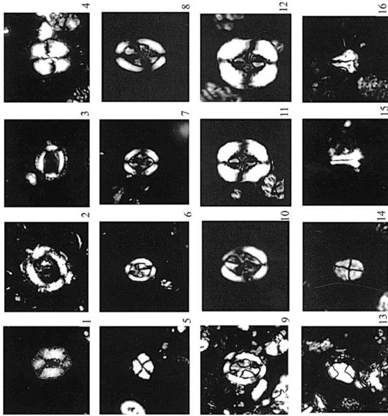
Fig. 1. Reticapsa ficula (stover, 1966) Burnett, 1998, XPL. Figs. 2-3. Manvitella pemmatoidea (Deflandre in Manivit, 1965) Thierstein, 1971, XPL. Fig. 4-5. Watznauria barnesae (Black in Black & Barnes, 1959) Perch - Nielsen, 1968, XPL. Figs. 6-7. Arkhangelskiella confusa Burnett, 1998, XPL. Figs. 8-9. Arkhangelskiella cymbiformis Vekshina, 1959, XPL. Fig. 10. Arkhangelskiella maastrichtiana Burnett, 1988, XPL. Figs. 11-12. Broinsonia parca parca Hattner et al., 1980, XPL. Figs. 13. Calculites obscurus (Deflandre, 1959) Prins & Sissingh in Sissingh, 1977, XPL. Fig. 14. Calculites ovalis (Stradner, 1963) Prins and Sissingh in Sissingh, 1977, XPL. Figs. 15-16. Lucianorhabdus maleformis Reinhardt, 1966, XPL. light microscope at X 2850 (XPL)
