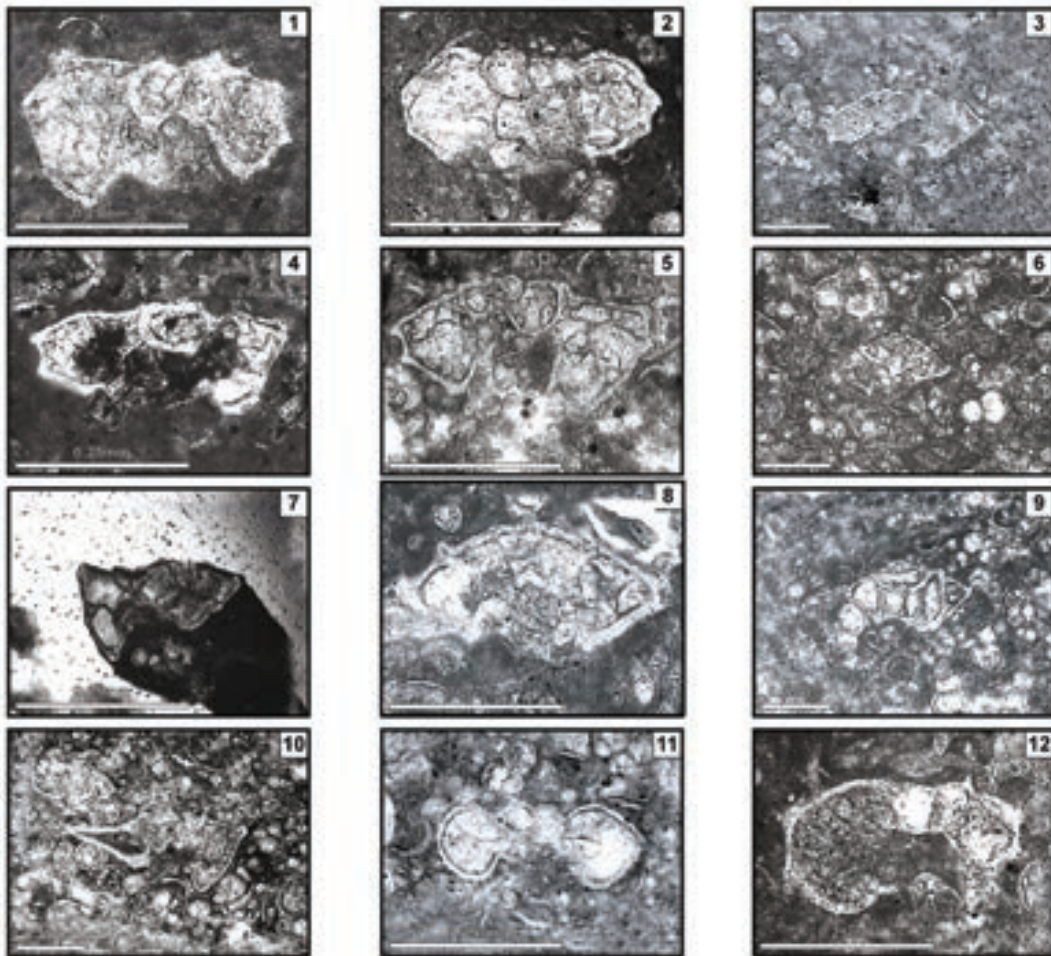
Fig 1. Globotruncana aegyptiaca , Sample No. Aks. 1799, Kuh-e Nareh Fig 2. Globotruncana bulloides , Depth: 1746m, Halegan well Fig 3. Globotruncana falsostuarti , Sample No. Aks. 1536, Kuh-e Ham Fig 4. Globotruncana Lapparanti , Sample No. Aks. 1793, Kuh-e Nareh Fig 5. Globotruncana ventricosa , Sample No. Aks. 1767, Kuh-e Nareh Fig 6. Globotruncanita conica , Sample No. Aks. 1800, Kuh-e Nareh Fig 7. Globotruncanita elevata , Depth: 1820m, Halegan well Fig 8. Globotruncanita stuarti , Sample No. Aks. 1544, Kuh-e Ham Fig 9. Globotruncanita stuartiformis , Sample No. Aks. 1540, Kuh-e Ham Fig 10. Radotruncanita calcarata , Sample No. Aks. 1794, Kuh-e Ham Fig 11. Globotruncanella havanensis , Sample No. Aks. 1533, Kuh-e Ham Fig 12. Archaglobiperina blowi , Sample No. Aks. 1527, Kuh-e Ham
