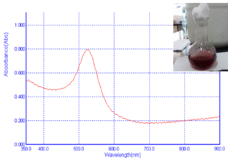
Fig. 2. UV-Vis spectrum of colloidal AuNPs. The absorption has been recorded from 350 to 900 nm. SPR peaks occurs at 524 nm.
