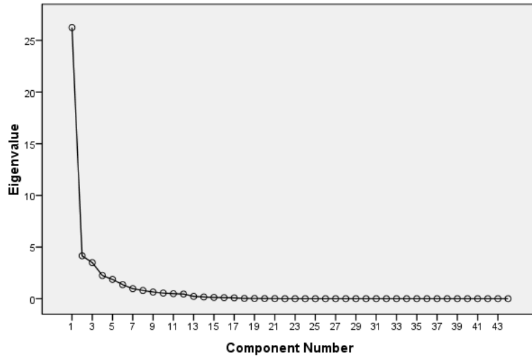
Scree Plot
