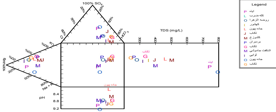
Durov Diagram
