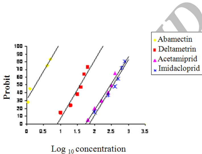
Figure 1- Comparison of the effect of Abamectin's LC 50 with other insecticides on first instar larvae of the leaf miner L. sativae
