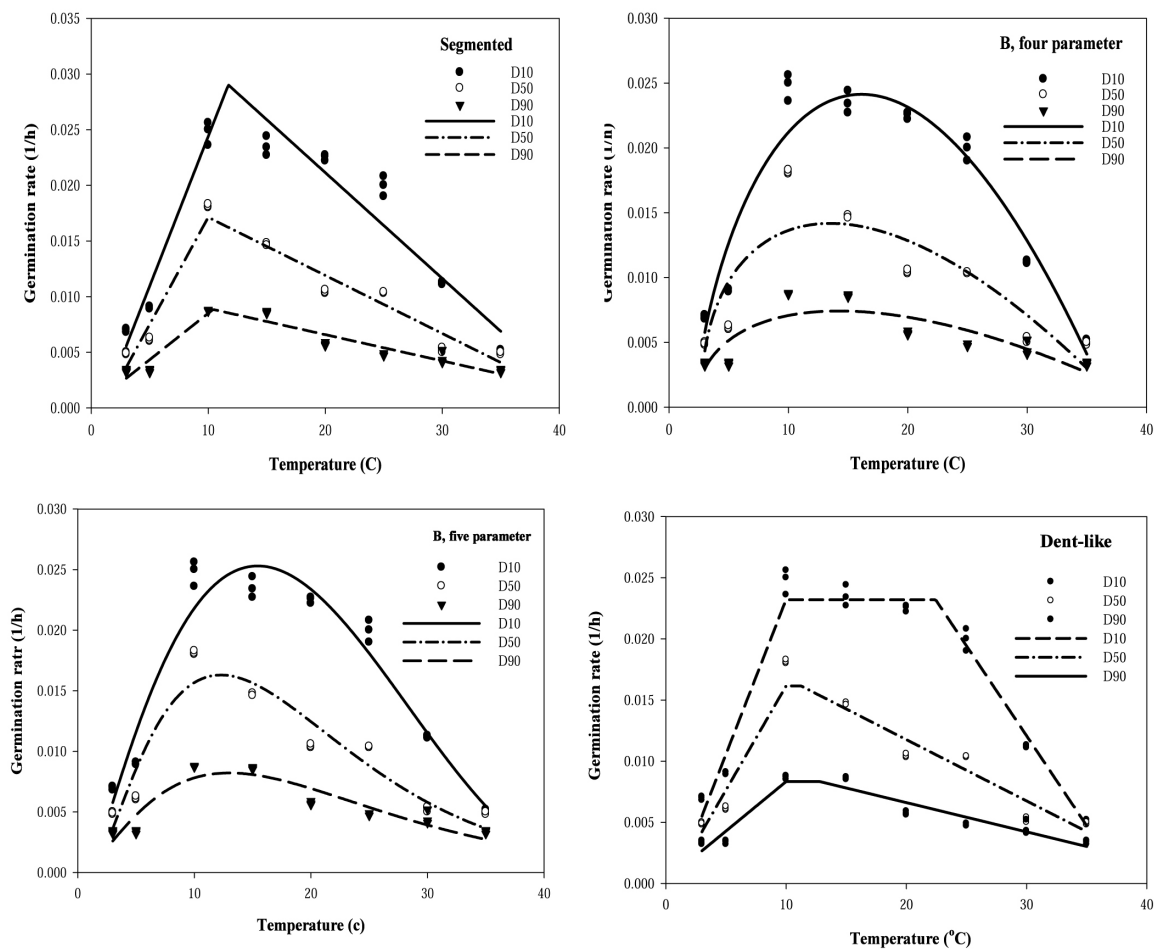
Figure 1- Predicted (lines) vs. observed (symbols) germination rates in Japanese Brome at constant temperatures for different germination percentiles (D 10 , D 50 and D 90 ) using segmented, beta (four and five parameter) and Dent-like models
