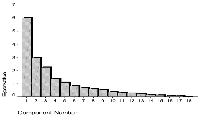
Scree Plot
