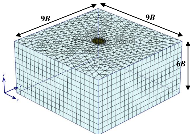
B=4, 2, 1 m
