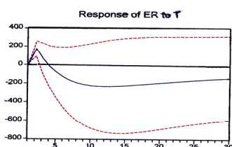
Response to One S.D. Innovations \pm 2 S.E.
