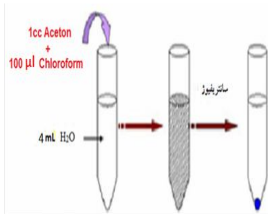
Fig 1 A simple schematic of Dispersive liquid-liquid microextraction
