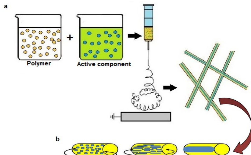
Fig 7 Schematic illustration of (a) emulsion electrospinning, (b) de-emulsification process of the polymeric emulsion under the influence of electrostatic charges during emulsion electrospinning.
