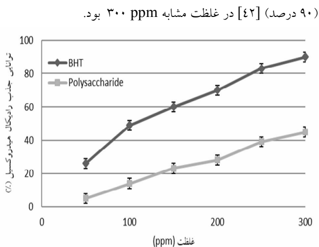
Fig 4 Capability of extracted soluble polysaccharide from Pleurotus ostreatus on scavenging of OH radicals at different concentrations
