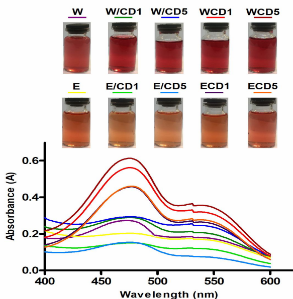
Fig 3 UV-Vis spectra of powder samples. W: water, E: Ethanol, BCD: \beta -cyclodextrin.
