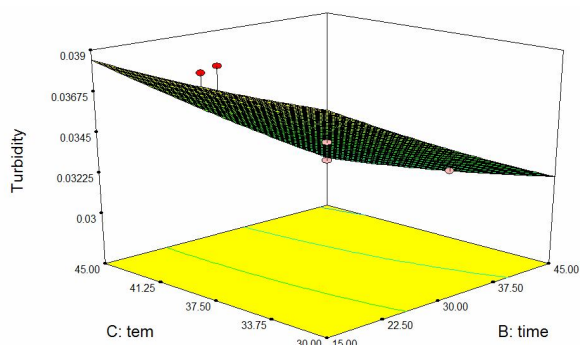
Fig 6 3D response surfaces changes the amount of turbidity by changing the temperature and time of the constant amount of enzyme 4 mg
