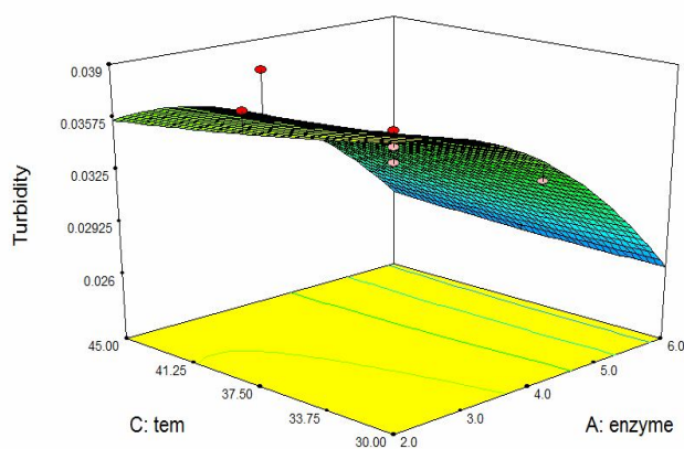
Fig 5 3D response surfaces changes the amount of turbidity by changing the temperature and enzyme level at a constant rate of 30 minutes
