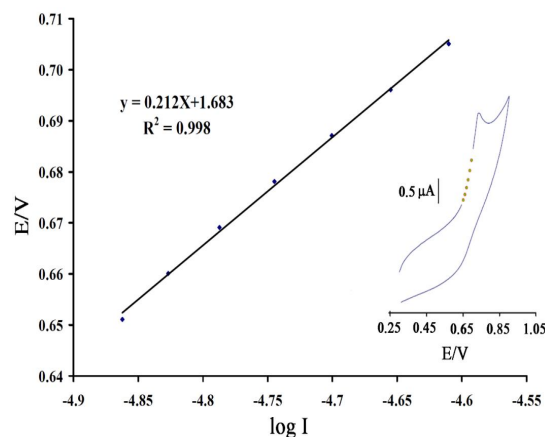
Fig 9 The Tafel plot obtained from cyclic voltammogram data of sunset yellow
