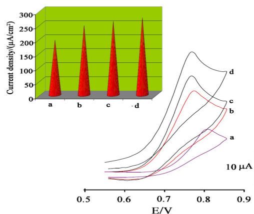
Fig 7 Cyclic voltammograms of (a) carbon paste electrode, (b) carbon paste electrode with graphene quantum dot nanoparticles, (c) carbon paste electrode with ionic liquid, (d) carbon paste electrode with ionic liquid and graphene doantom dot nanoparticles in presence of 250 \mu\text{M} sunset yellow. Inset: the current density derived from cyclic voltammograms
