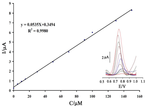
Fig 11 The plot of peak current as a function of sunset yellow concentrations at the modified graphene-quantum dot nanoparticle electrode insert: the square wave voltammograms of midified electrode in presence of various sunset yellow concentrations in the range of 3 nM to 150 μM
