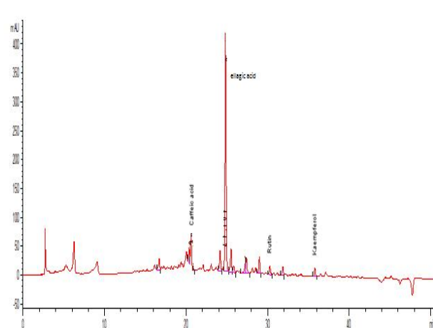
Fig 1 Coromatogram Diagram (HPLC) eucalyptus extract to identify effective compounds
