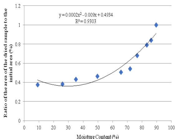
Fig 3 Changes in the surface area of dried beetroot at 60 °C compared to the initial area.
