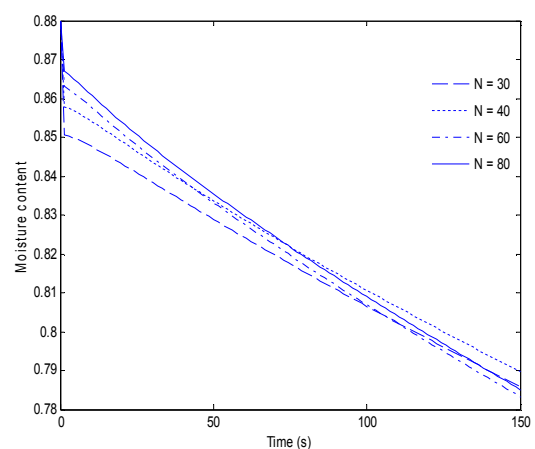
Fig 6 mesh independence
