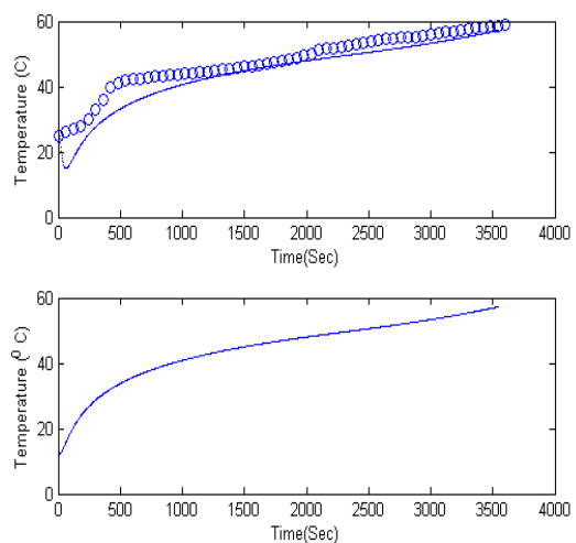
Fig 13 Sample temperature changes during drying at 70 °C.
