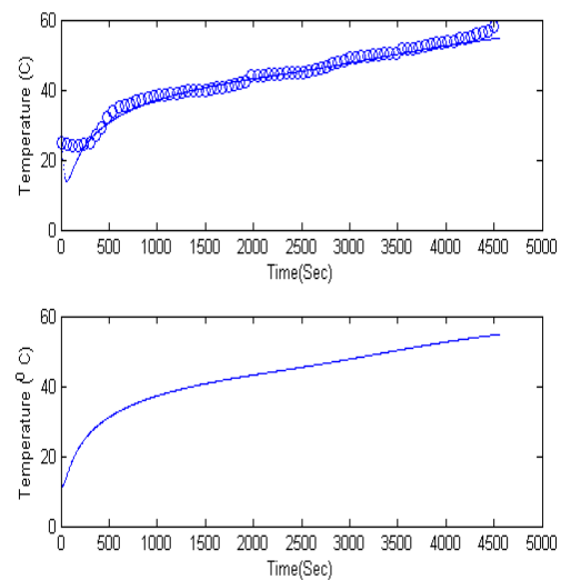
Fig 12 Sample temperature changes during drying at 60 °C.
