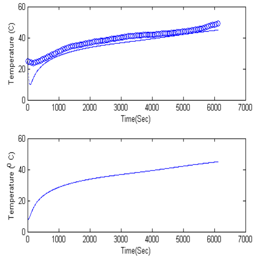
Fig 11 Sample temperature changes during drying at 50 °C
