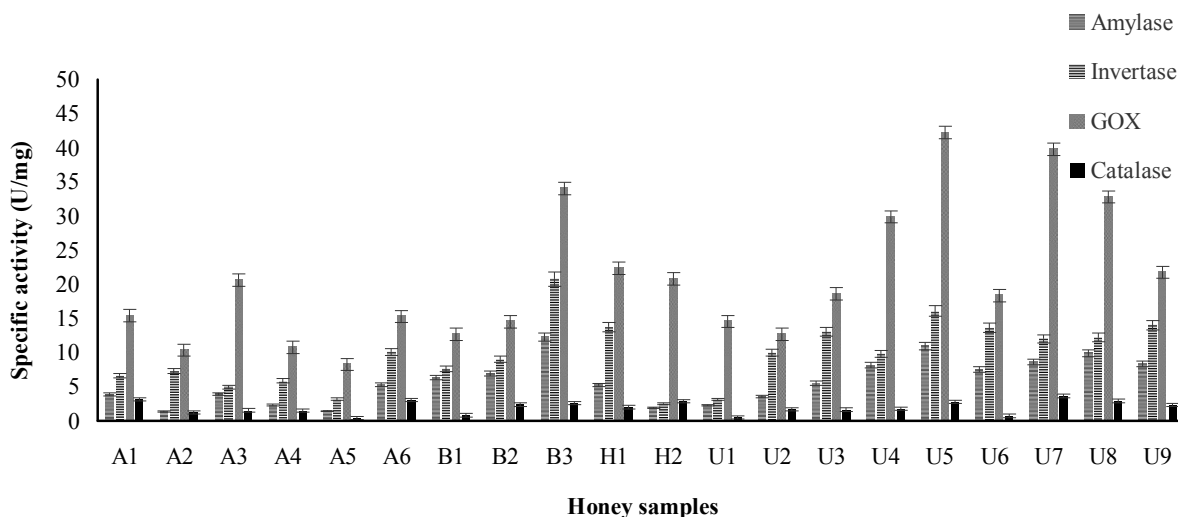
Fig 2 Specific activity of amylase, invertase, glucose oxidase, and catalase enzymes ( \mu\text{mole min}^{-1} \text{mg}^{-1} \text{protein} ) in protein solution of 20 Iranian honey samples.
