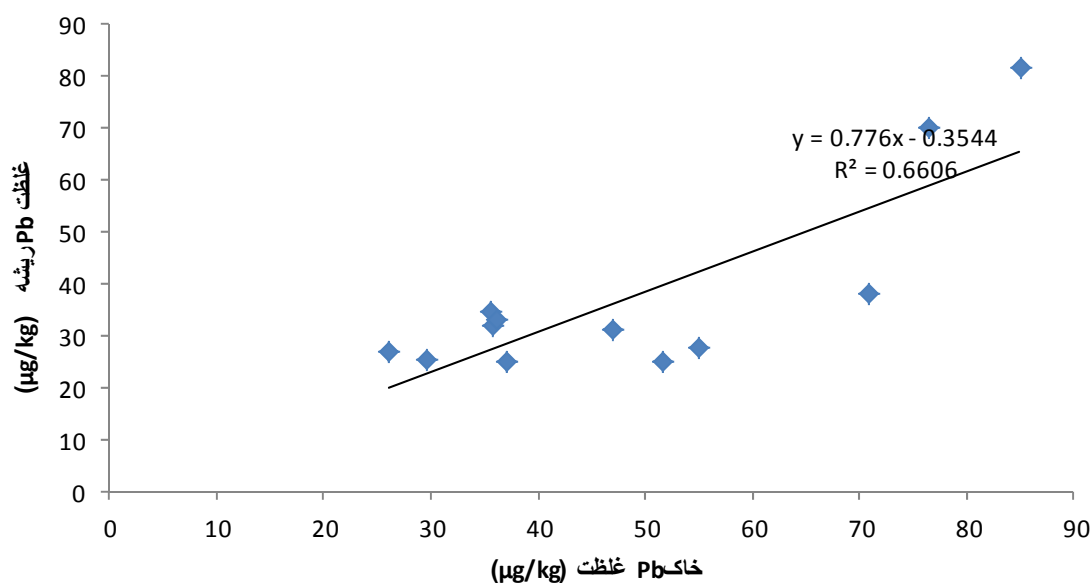
Diagram 2-The correlation between Pb concentrations in soil with root
