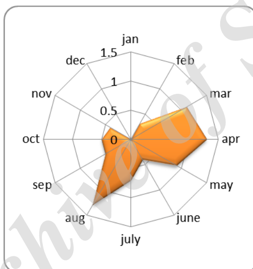
Figure 5. The monthly average changes of dust storms in Nahavand station (1996 -2005)
