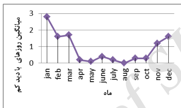
Figure 9. The monthly average of days with visibility less than 2 kilometers in Malayer station (1992-2010)
