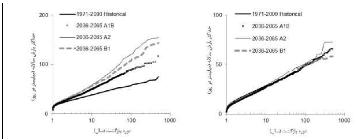
Fig. 4- Climate change impact on maximum daily rainfalls
