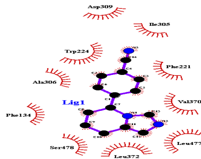
Fadrozole_Complex
