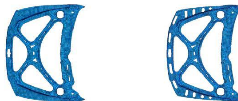
FE model of the former inner panel b FE model of the new inner panel
