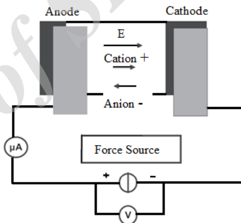
Fig. 1 General schematic for electroplating process
