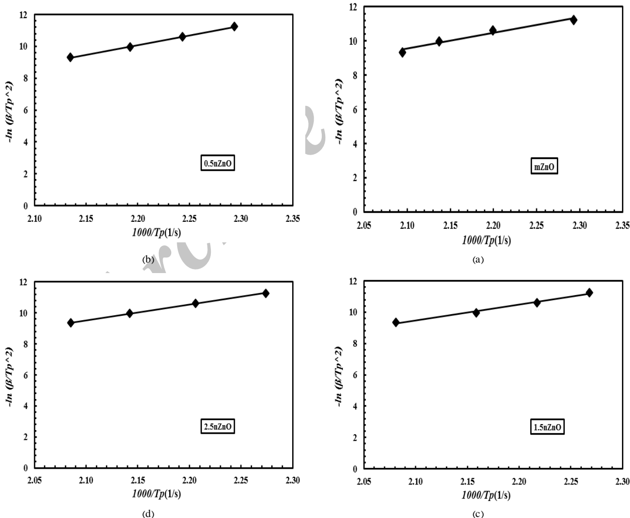
Fig. 6 Kissinger plot for pure sample (a), sample with 0.5 phr ZnO (b), sample with 1.5 phr ZnO (c) and sample with 2.5 phr ZnO (d)
