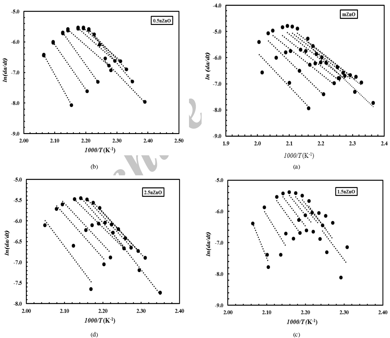
Fig. 8 Plot of \ln(da/dt) vs. 1/T for control system (a), sample with 0.5 phr ZnO (b), sample with 1.5 phr ZnO (c) and sample with 2.5 phr ZnO (d)
