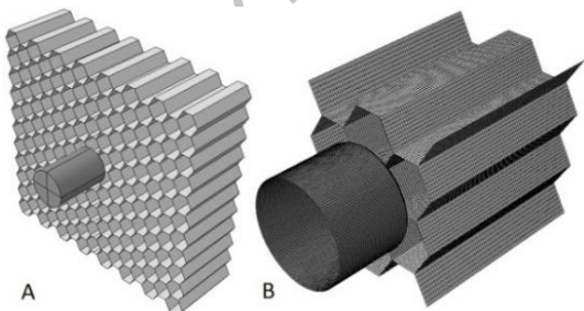
Fig. 3 A) Geometrical model for collision of flat projectile with honeycomb B) mesh around the collision region
