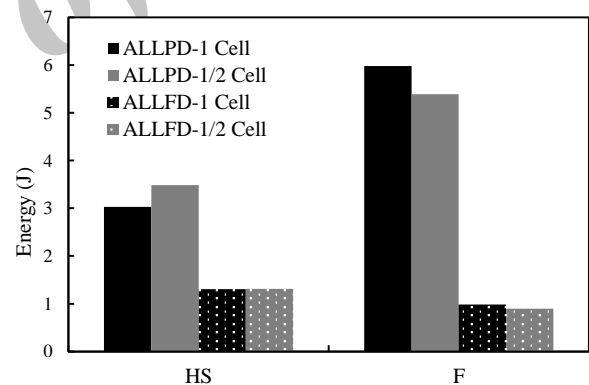
Fig. 19 Plastic (ALLPD) and frictional dissipated energy (ALLFD) in models with different honeycomb cell dimensions
