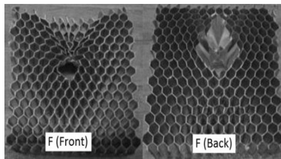
Fig. 16 Front and Back views of honeycomb after F projectile collision [16]
