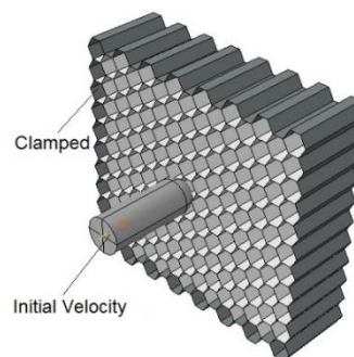
Fig. 4 Honeycomb and projectile boundary conditions
