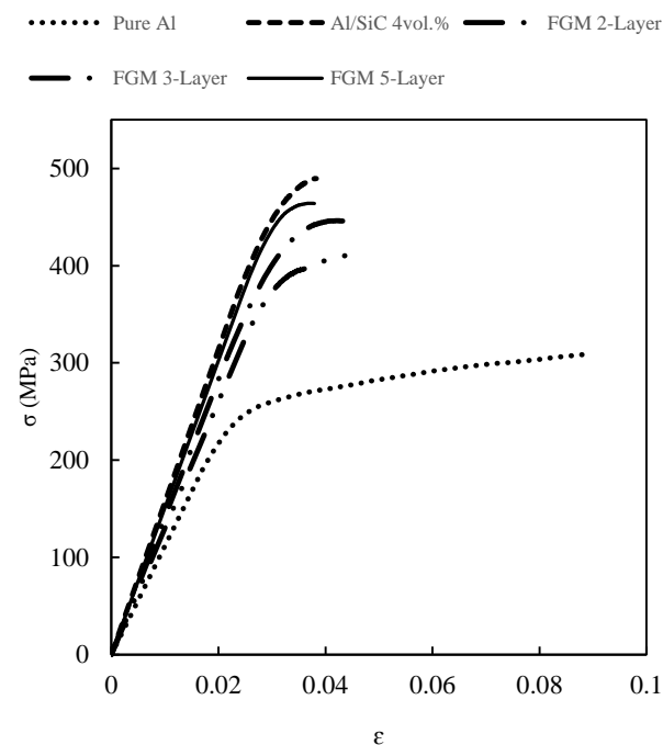
Fig. 17 Engineering tensile stress-strain diagram for pure, composite and FGM samples
