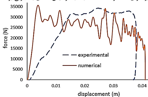
Fig. 13 Comparison of Force- Displacement diagram of experimental and numerical results in the samples with 30mm diameter
