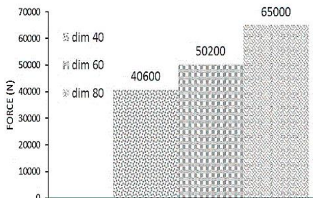
Fig. 17 Force value in first area in different diameter of sample
