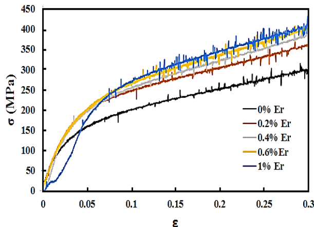
Fig. 9 Compressive stress-strain curves of modified Al-15%Mg 2 Si composite with various amounts of Er.
