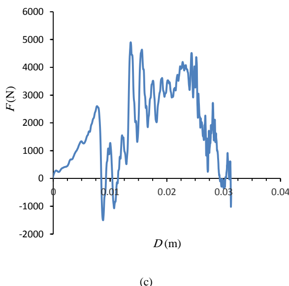
Fig. 7 Force-Displacement diagram for 60 J impact test a: T1, b: T2, c: T3
