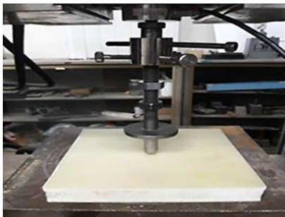
Fig. 2 Applying pressure force to the sandwich panel in a static pressure test
