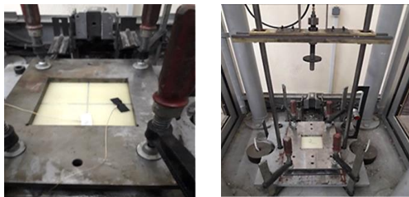
Fig. 3 Impact test device with clamping sandwich panel in its position
