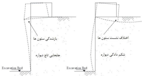
Fig. 3. Effect of wall deformation on damage type of adjacent structure
