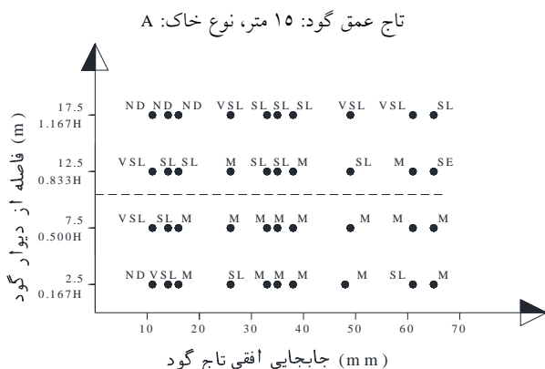
Fig. 12. Damage level based on horizontal displacement of excavation wall Excavation depth: 15m, Soil type: A
