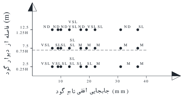
Fig. 13. Damage level based on horizontal displacement of excavation wall Excavation depth: 10m, Soil type: A
