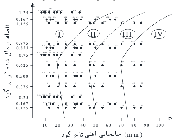
Fig. 14. Damage levels, Soil type: A
