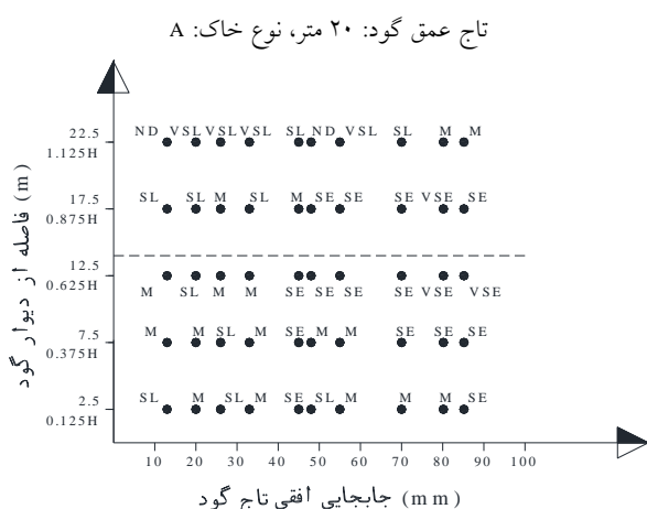
Fig. 11. Damage level based on horizontal displacement of excavation wall Excavation depth: 20m, Soil type: A
