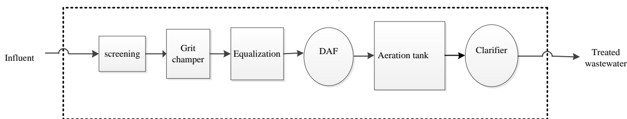
Fig 1. Flow diagram of ABS wastewater treatment plant
