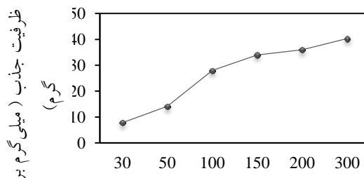
Figure (4): The effect of concentration on adsorption of MB onto PS (0.07g/20ml) at pH of 7 and tem. of 25±2°C
