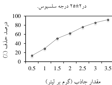
Figure (3): The effect of dosage on adsorption of MB(100mg/l) at 25±2°C
