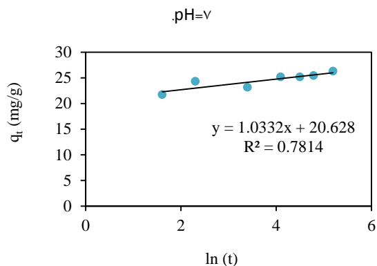
Figure (9): Elovich kinetic model of adsorption of MB onto PS (3.5g/l) at pH of 7
