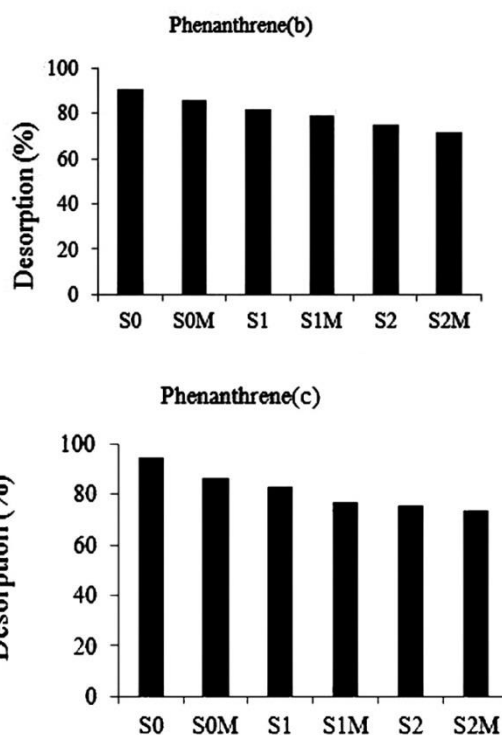
Fig. 4. Desorption of phenanthrene from soils a- back ground solution 0.01M CaCl 2 b- back ground solution 0.01M EDTA and 7.5 Tween 80 c- background solution 0.01M EDTA and 7.5 Triton X100
