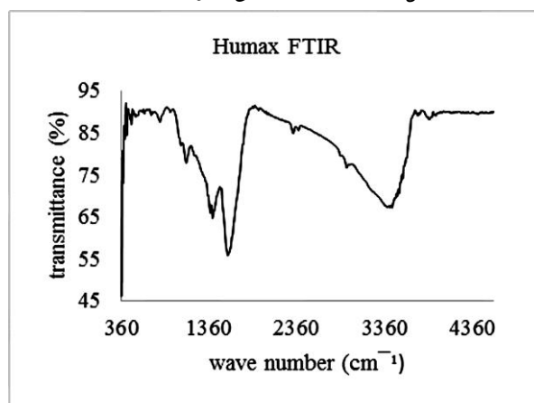
Fig. 2. FTIR spectrum of organic matter
