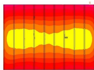
Fig. 17. Lateral displacement of ordinary jack arch roof
