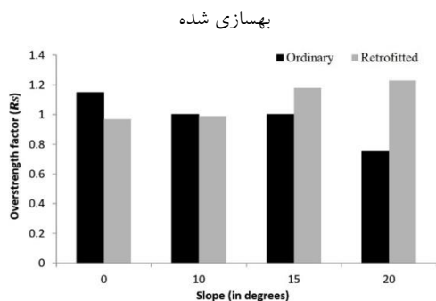
Fig. 26. Overstrength factor R_s for ordinary and retrofitted structures
