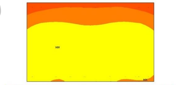
Fig. 18. Lateral displacement of retrofitted jack arch roof
