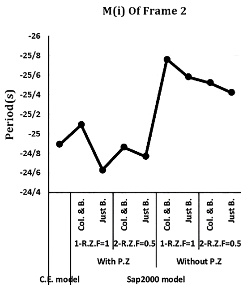
Fig. 25. Moment in node (i) of frame 2
