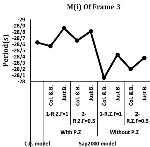
Fig. 26. Moment in node (i) of frame 3
