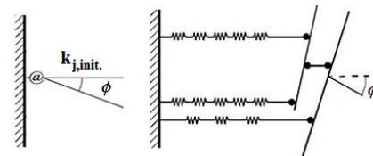
Fig. 2. EC Model of Semi Rigid Connection (Right)-Simplified Model of EC (Left)
