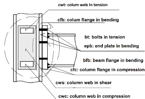
Fig. 1. Effective components in end plate connection
