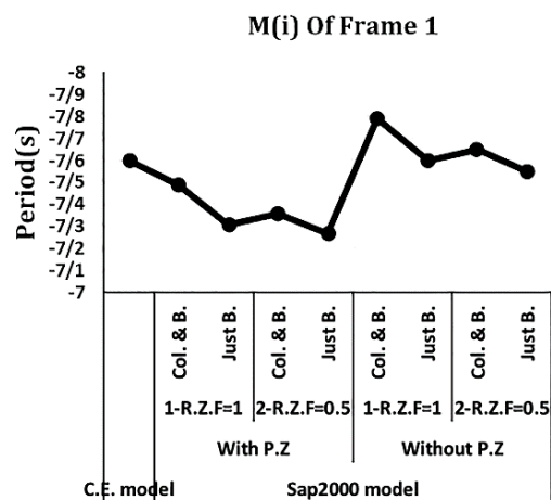
Fig. 24. Moment in node (i) of frame 1
