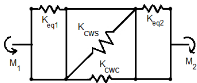
Fig. 3. EC Model for End Plate Connection
