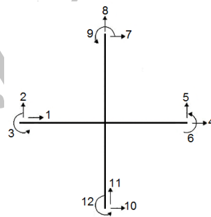
Fig. 4. Cruciform Element of Connection
