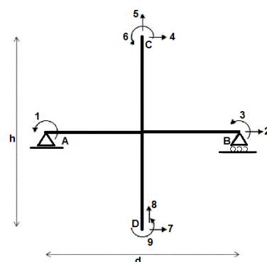
Fig. 5. Stability Model of Cruciform Element
