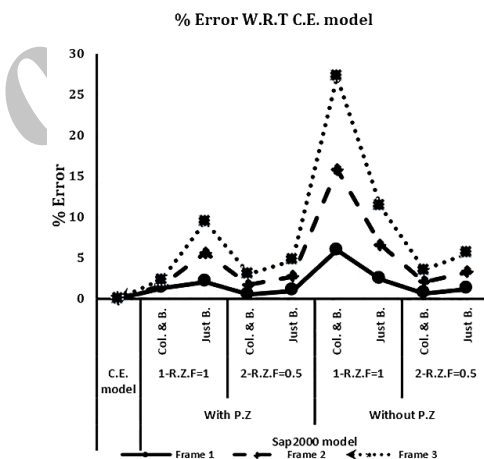
Fig. 15. Main period difference in all models with C.E Model
