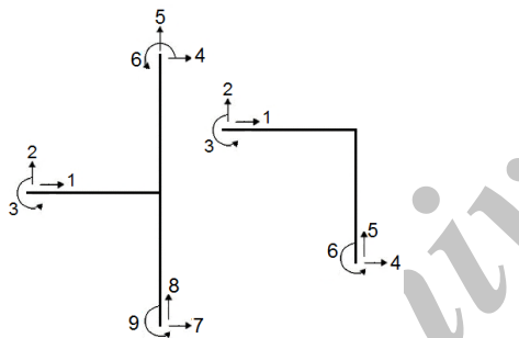
Fig. 7. Two Models of Corner Connections and Degree of Freedom's
