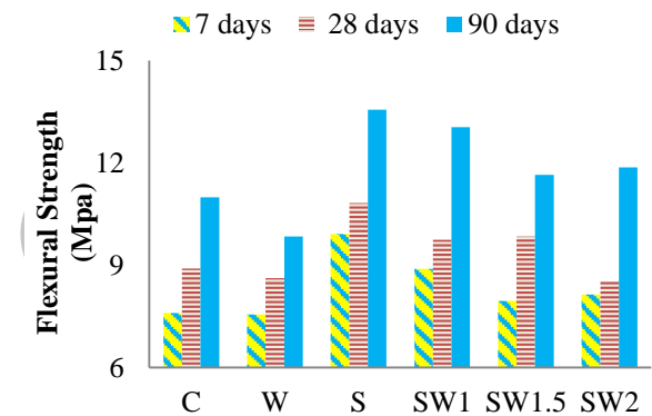
Fig. 10. Flexural strength of concrete with steel fibers and sealing material (bc39)
