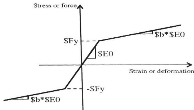
Fig. 2. Steel 01 Material
