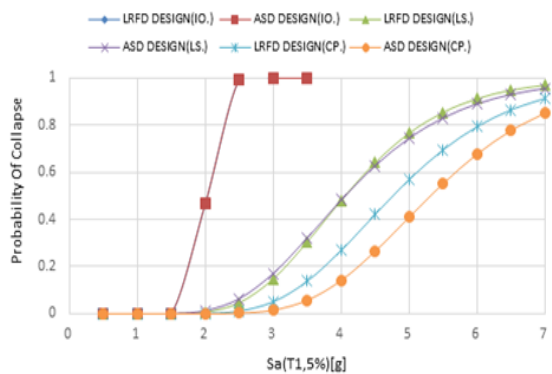
Fig. 13. Fragility Curve for 8- Story Intermediate Moment Frame
