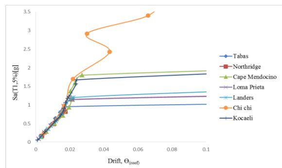
Fig. 3. IDA Curve Of Four- Story IMF (ASD. Method)
