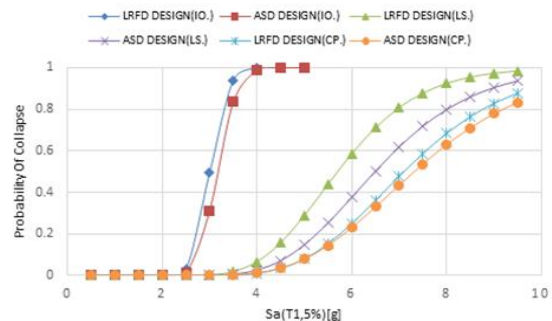
Fig. 12. Fragility Curve for 4- Story Special Moment Frame
