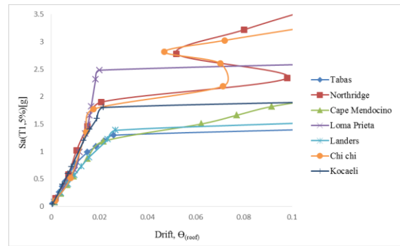
Fig. 9. IDA Curve Of Eight- Story SMF (ASD, Method)
