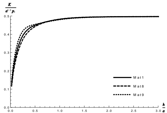
Fig. 10. The effect of \nu on the shearing stress intensity factor
