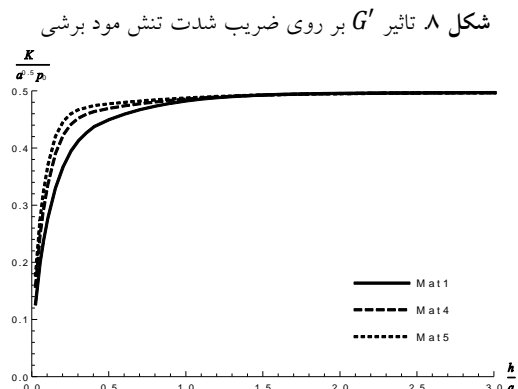
Fig. 8. The effect of G' on the shearing stress intensity factor
