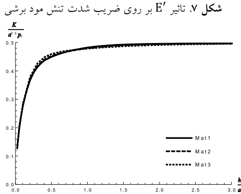
Fig. 7. The effect of E' on the shearing stress intensity factor
