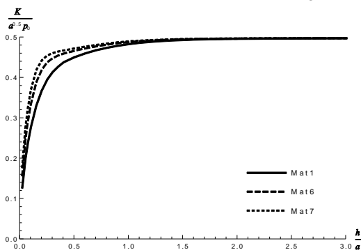
Fig. 9. The effect of E on the shearing stress intensity factor
