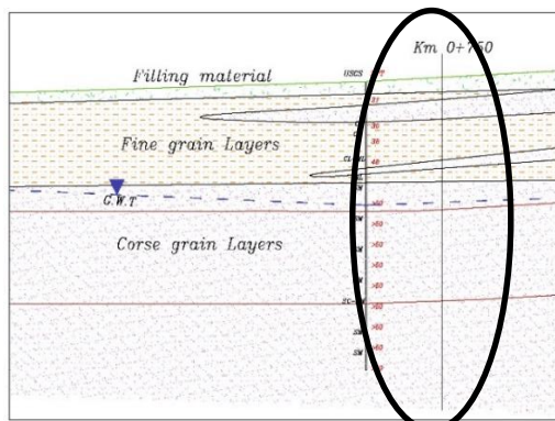
Fig. 2. Geological profile of Tabriz metro line 2 at KM +0.750
