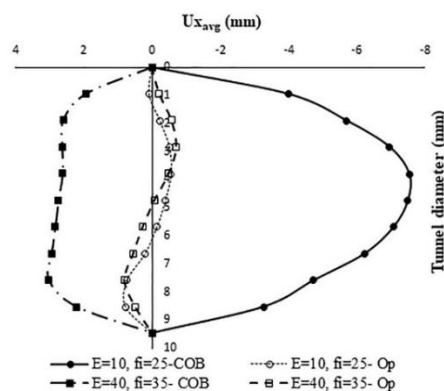
Fig. 4. horizontal displacement at face
