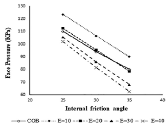
Fig. 7. Variation of internal friction angle- face pressure
