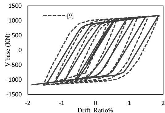
Fig. 6. Comparing numerical results to those of Berman and Bruneau (2007).
