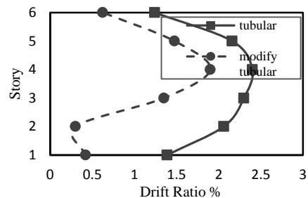
Fig. 10. The effect of cross-section in flexural link beams subjected to far-fault records
