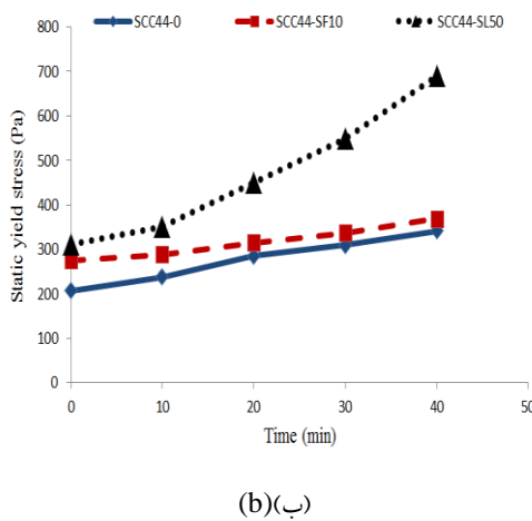
Fig. 3. Static yield stress changes for mixtures in 40 minutes with, (a) w/p of 0.42, (b) w/p of 0.44
