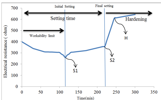
Fig. 4. Schematic behavior of concrete and mortar during time in E.R. test
