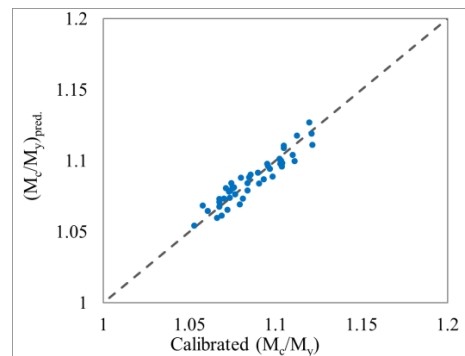
Fig. 11. Predicted/Calibrated Values for ( M_c/M_{y,p} )
